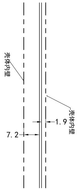
SA-016线-PCB
